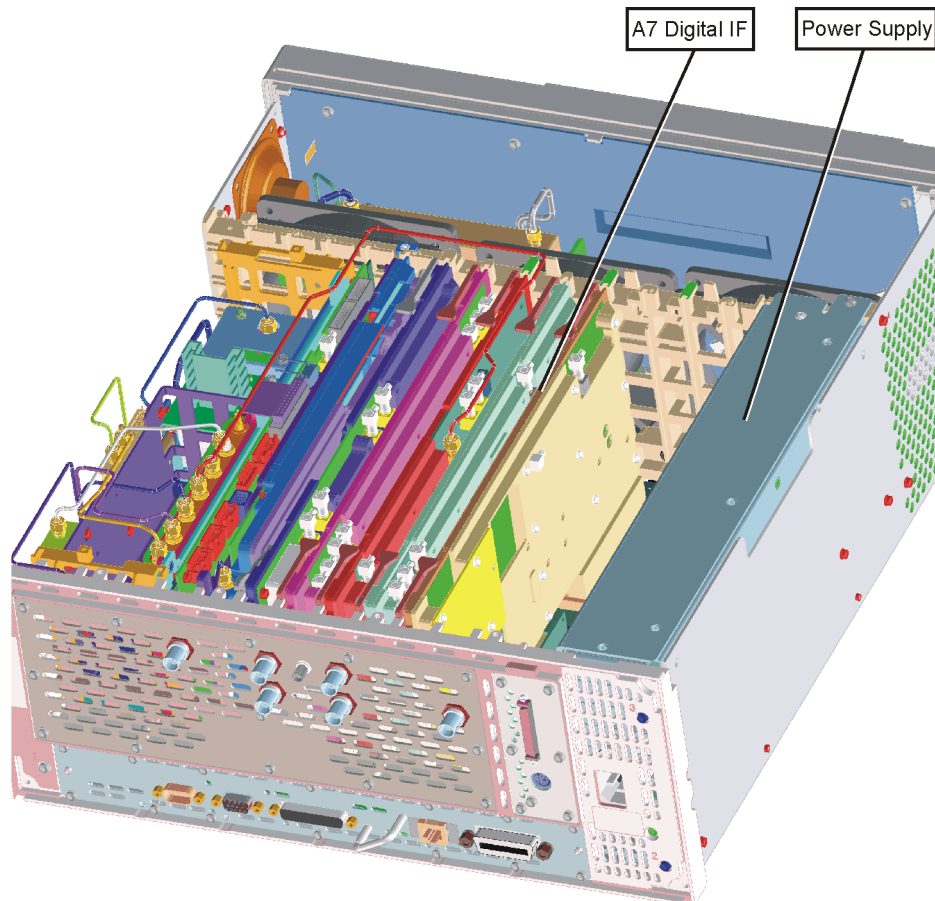
Figure 3 A7 Digital IF Assembly
